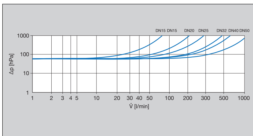
Fig. 3: Performance diagram pressure loss backflow preventer press/threaded connection
