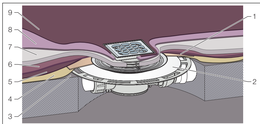
Fig. 7: Layer structure of the self-levelling coating
