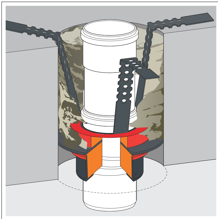
Fig. 5: Example: fire protection pipe lead-in
