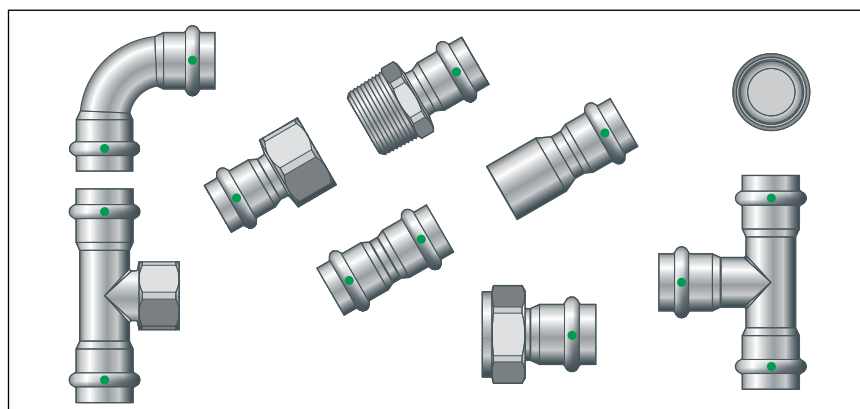
Fig. 1: Sanpress Inox press connectors
