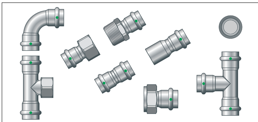
Abb. 1: Sanpress Inox-Pressverbinder
