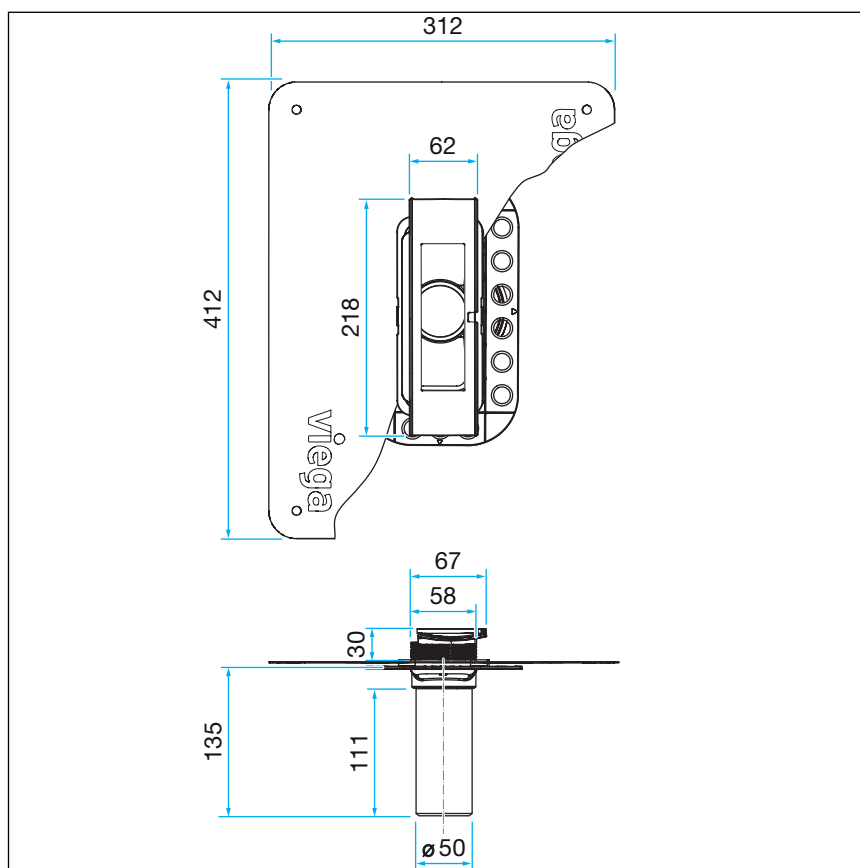
Fig. 3: Dimensions of base unit basic model
