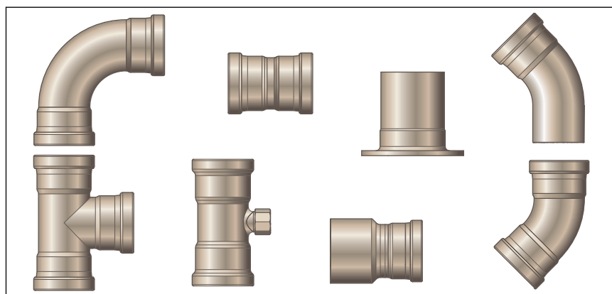
Fig. 1: Seapress XL – Overview
