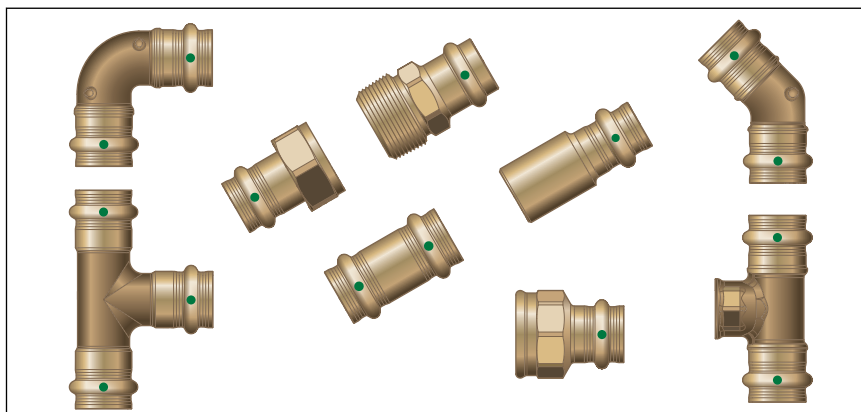
Abb. 1: Sanpress-Pressverbinder
