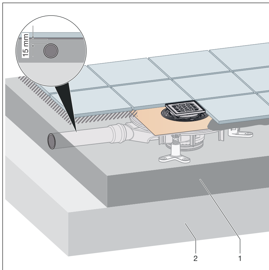
Fig. 9: Screed thickness, normal installation situation
