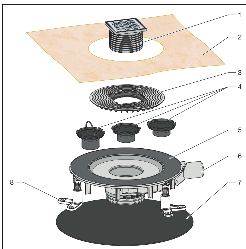
Fig. 1: Scope of delivery model 4914.20
