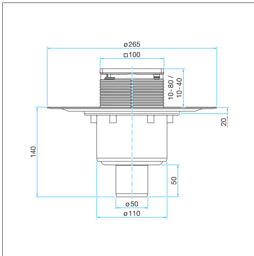
Fig. 7: Dimensional drawing for model 4936.3
