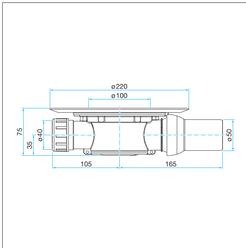
Fig. 8: Dimensional drawing model 4935.2
