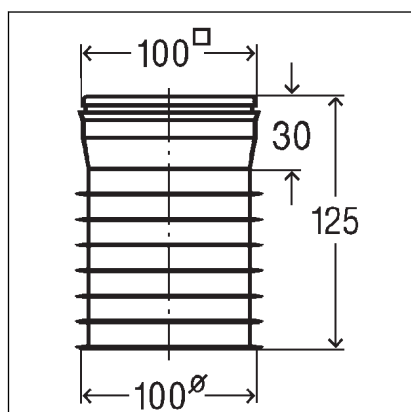
Fig. 3: Dimensional drawing
