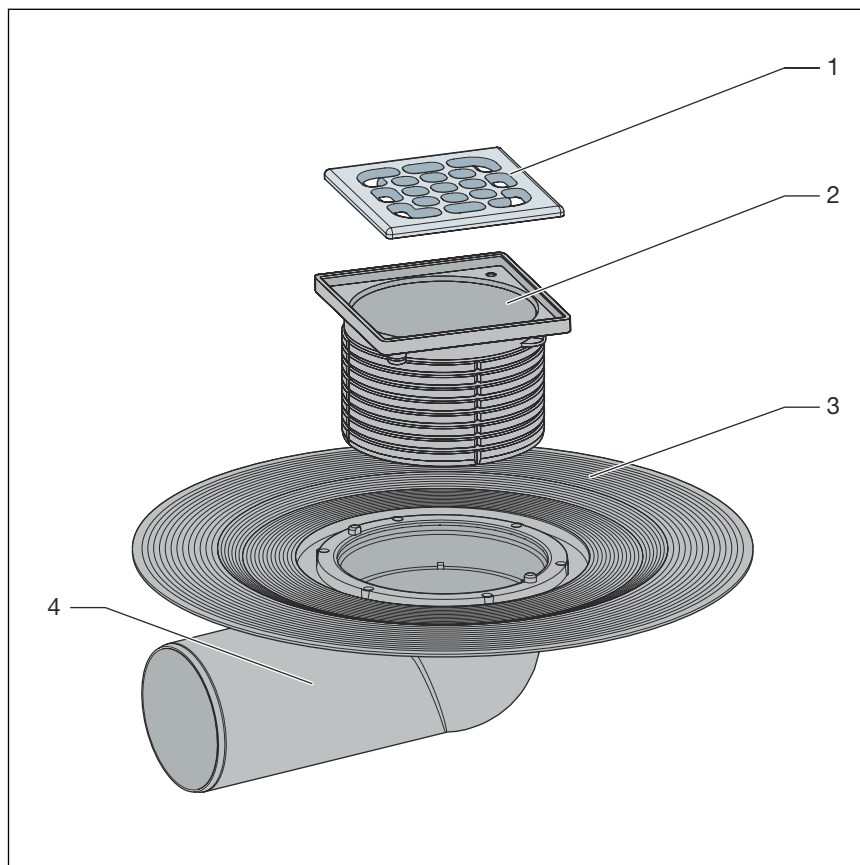
Fig. 1: Components balcony / terrace drain model 4943.2
