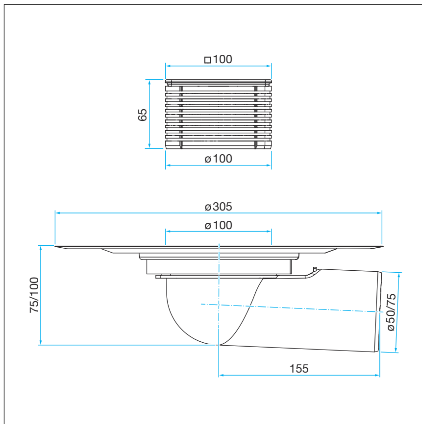
Fig. 7: Dimensional drawing for model 4943.2
