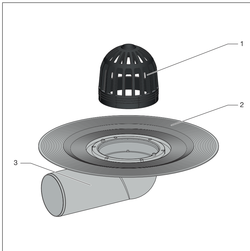
Fig. 1: Components balcony / terrace drain model 4945.2
