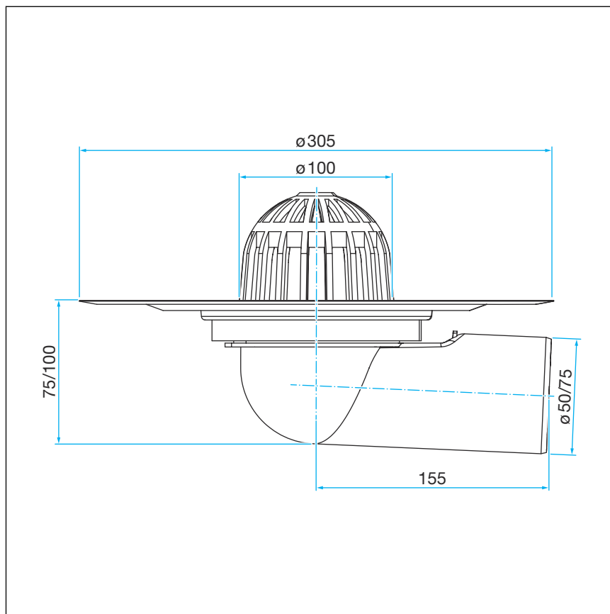
Fig. 5: Dimensional drawing for model 4945.2
