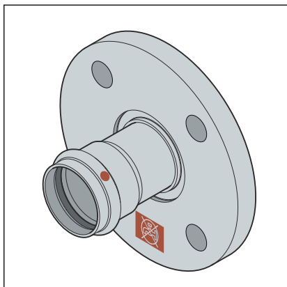
Fig. 11: Bride fixe
