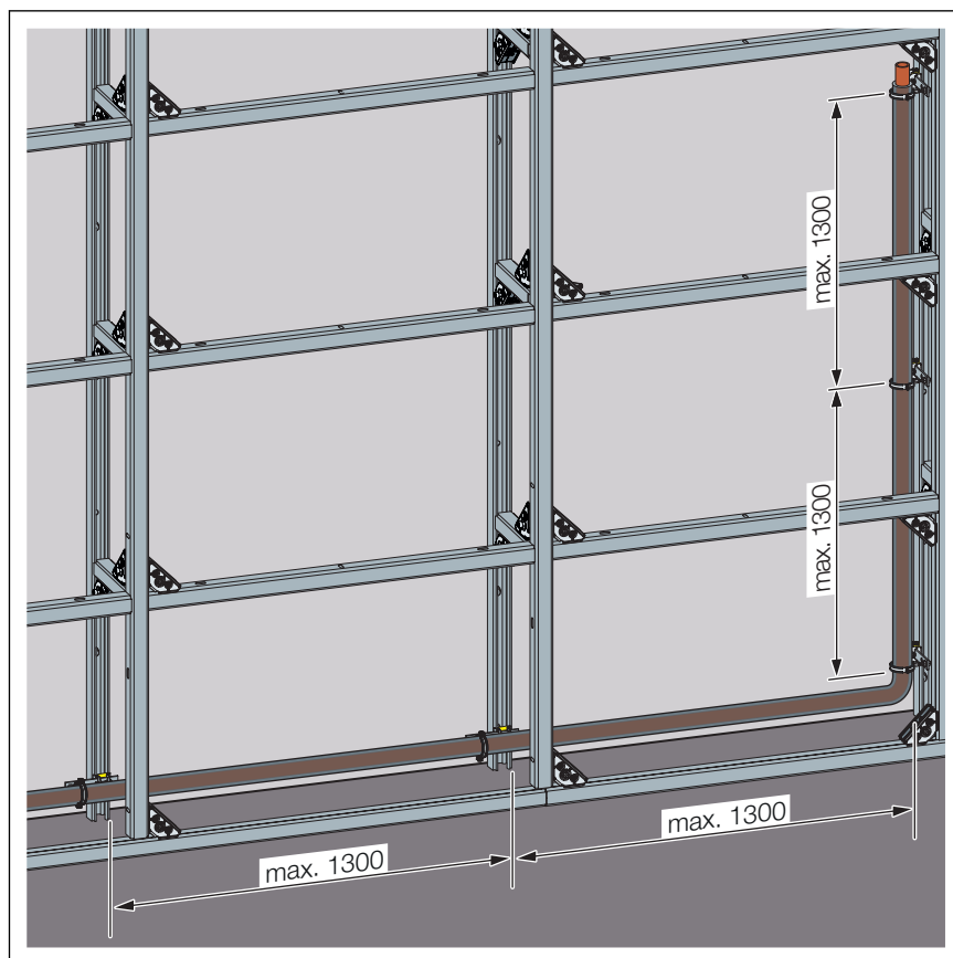
Fig. 4: Fixing distances
