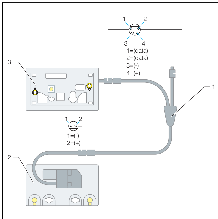
Fig. 2: Connection diagram, WC installation frame for Prevista
