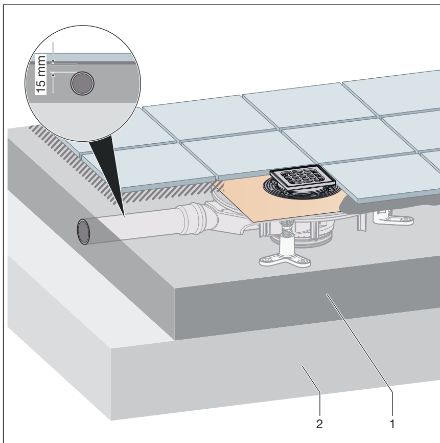
Fig. 9: Screed thickness, normal installation situation
