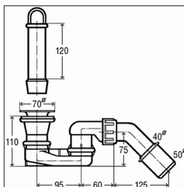
Fig. 2: Dimensional drawing
