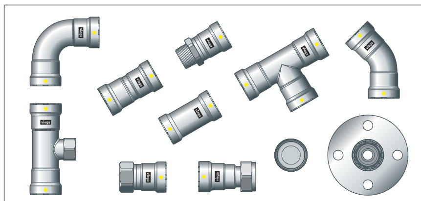
Afb. 1: Megapress G-persfittingen
