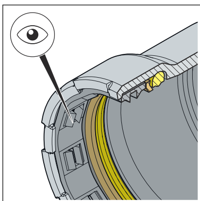
Afb. 9: Snijring
