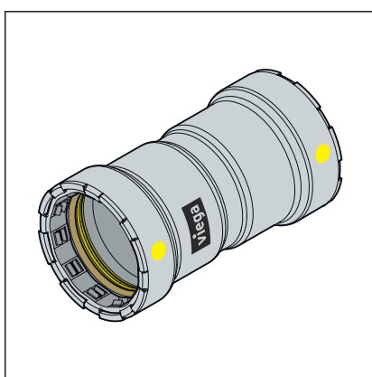
Abb. 2: Megapress G-Pressverbinder
