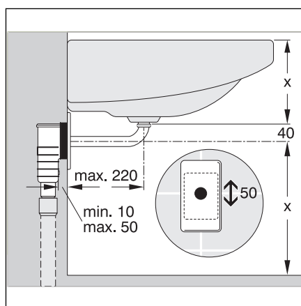
Fig. 3: Installation dimensions
