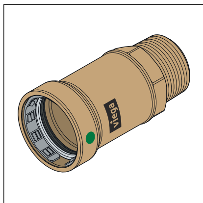
Fig. 2: Megapress adapter (model 4211.4)
