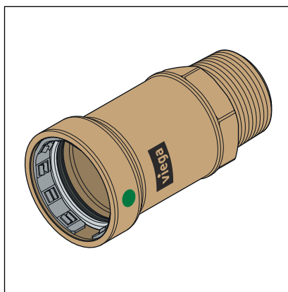
Fig. 1: Megapress adapter to R-thread (model 4211.4)
