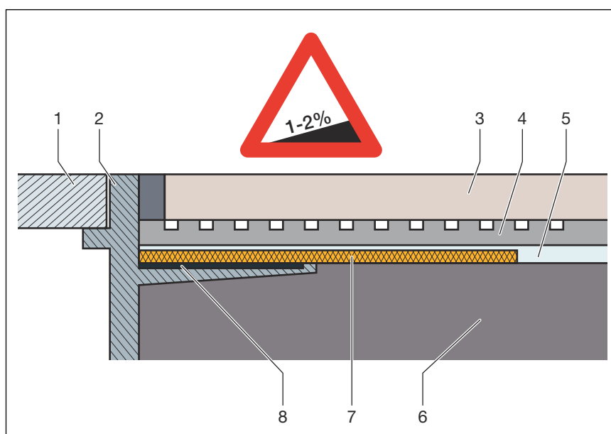
Fig. 7: Construction diagram of the bonded seal - min. screed incline 1–2 %
