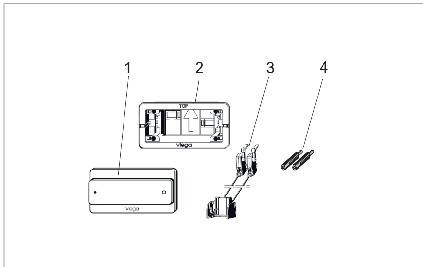
Fig. 1: Component overview
