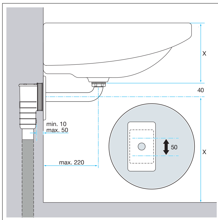
Fig. 3: Installation dimensions
