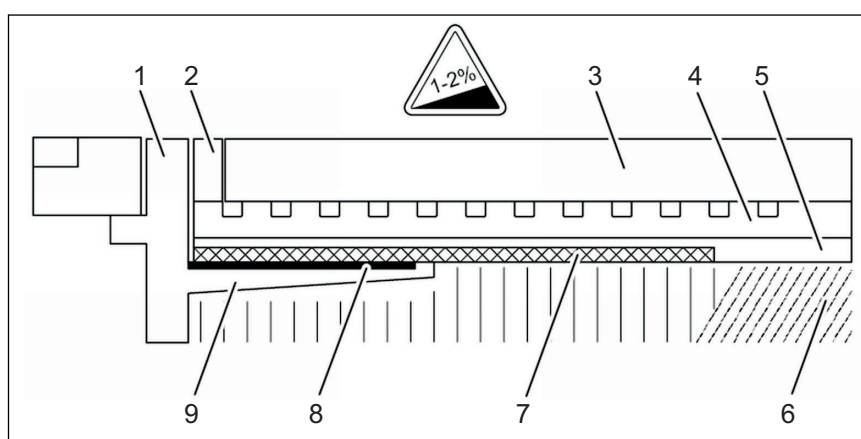
Fig. 2: Construction diagram of the bonded seal - min. screed incline 1–2 %
