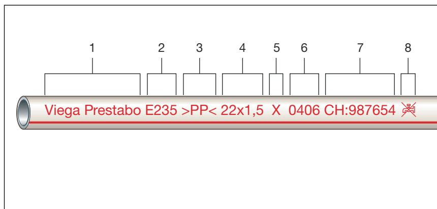
Abb. 7: Rohr PP-ummantelt
