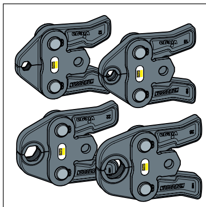
Abb. 8: Pressbacken
