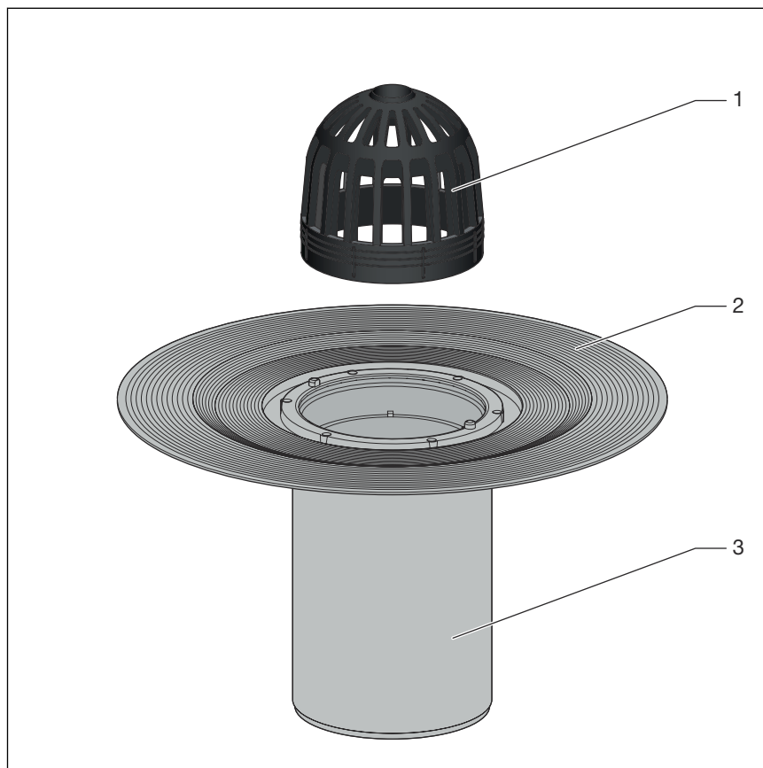
Fig. 1: Components balcony / terrace drain model 4946.2
