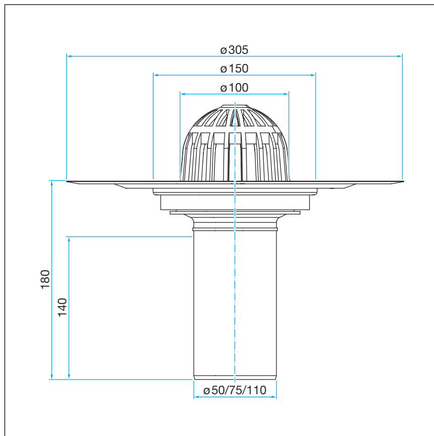
Fig. 5: Dimensional drawing for model 4946.2
