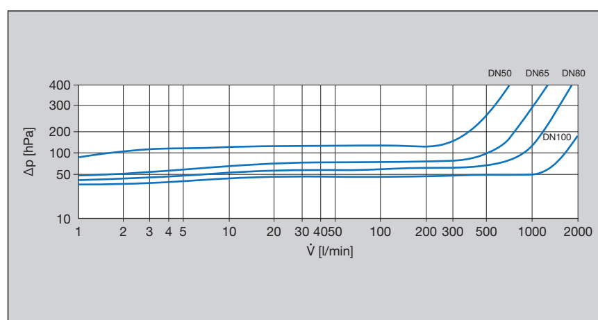
Fig. 1: Performance diagram pressure loss backflow preventer flange connection
