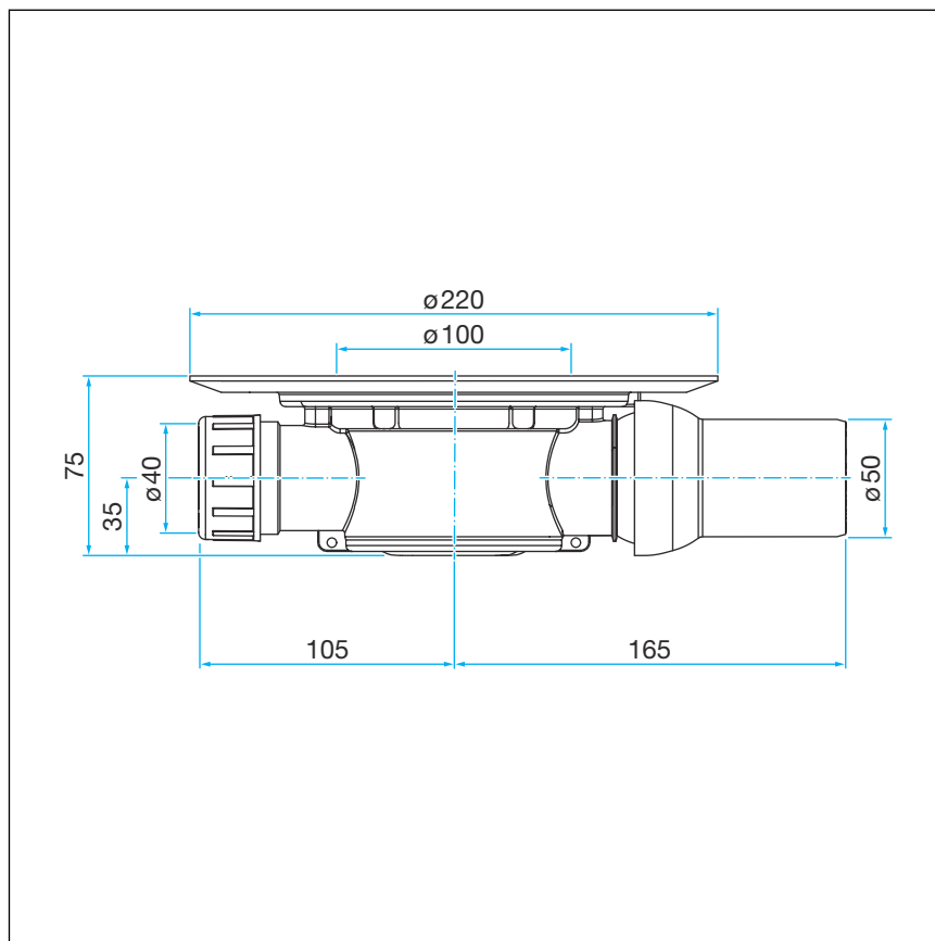
Fig. 8: Dimensional drawing model 4935.6
