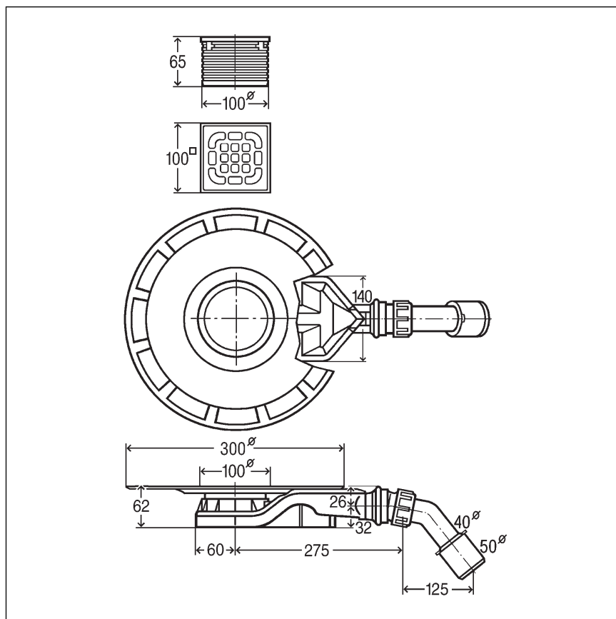
Fig. 6: Dimensional drawing model 4980.60
