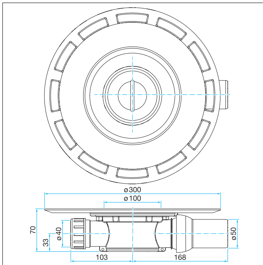
Fig. 7: Dimensional drawing model 4938
