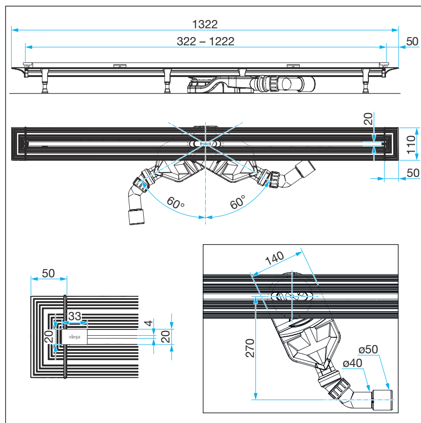
Fig. 13: Dimensions of base unit basic model
