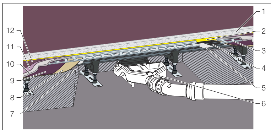
Fig. 20: Layer structure of the self-levelling coating
