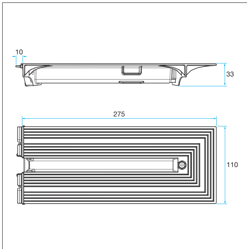
Fig. 15: Dimensions of end closing piece
