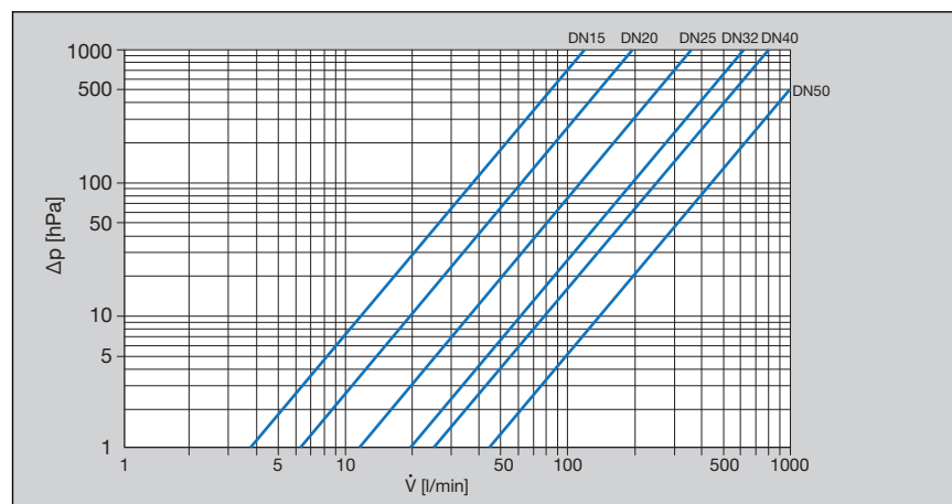
Fig. 1: Performance diagram slanted seat valve press/threaded connection
